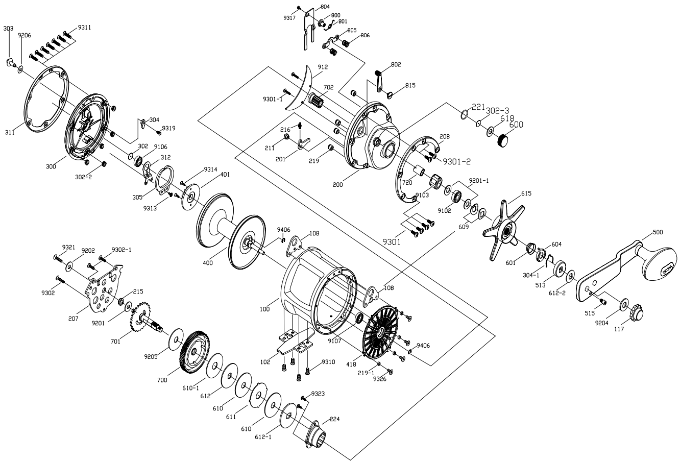
CT - 55W Spare Parts
